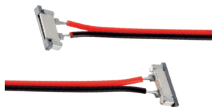
ACC02 One colour LED strip connector, 150mm cable
