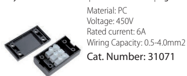
Terminal box IP44
